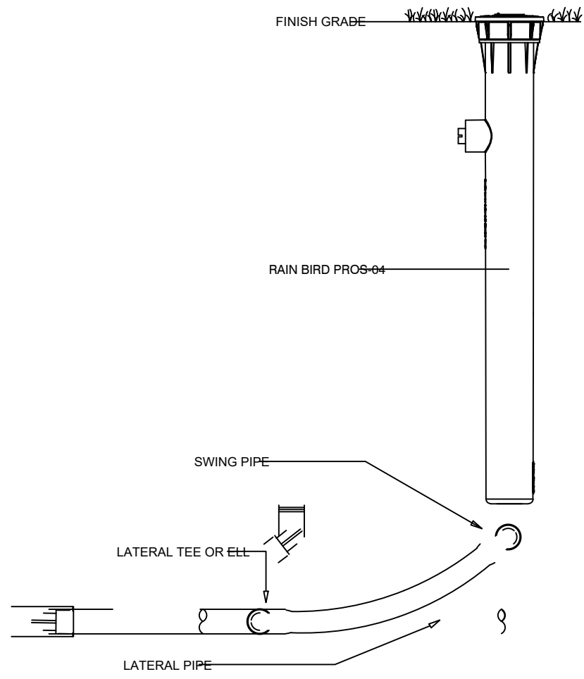
1 POP-UP SPRAY SPRINKLER
