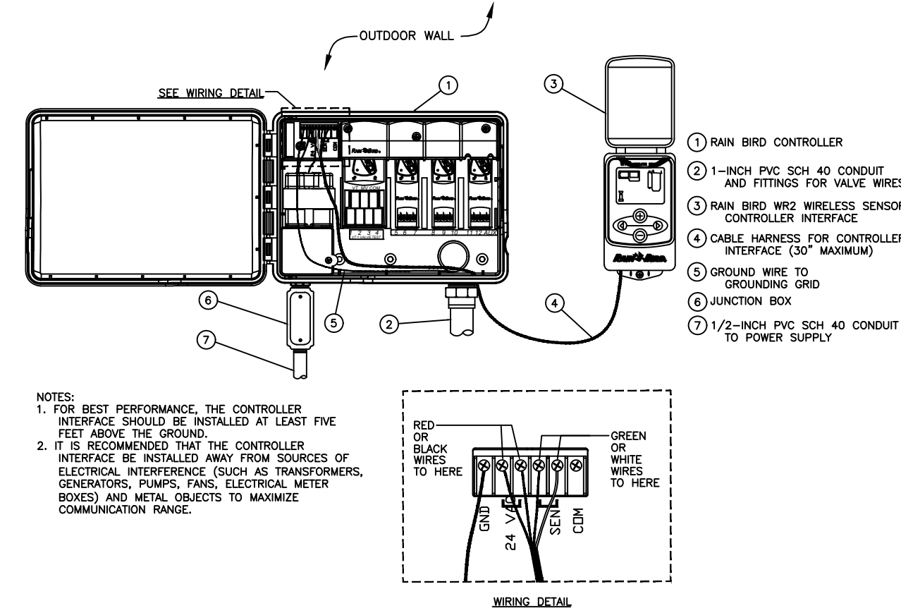
6 WR2 WIRELESS RAIN SENSOR
