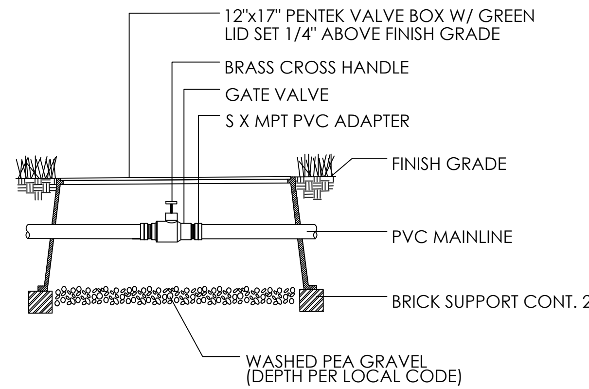
3 ISOLATION VALVE
